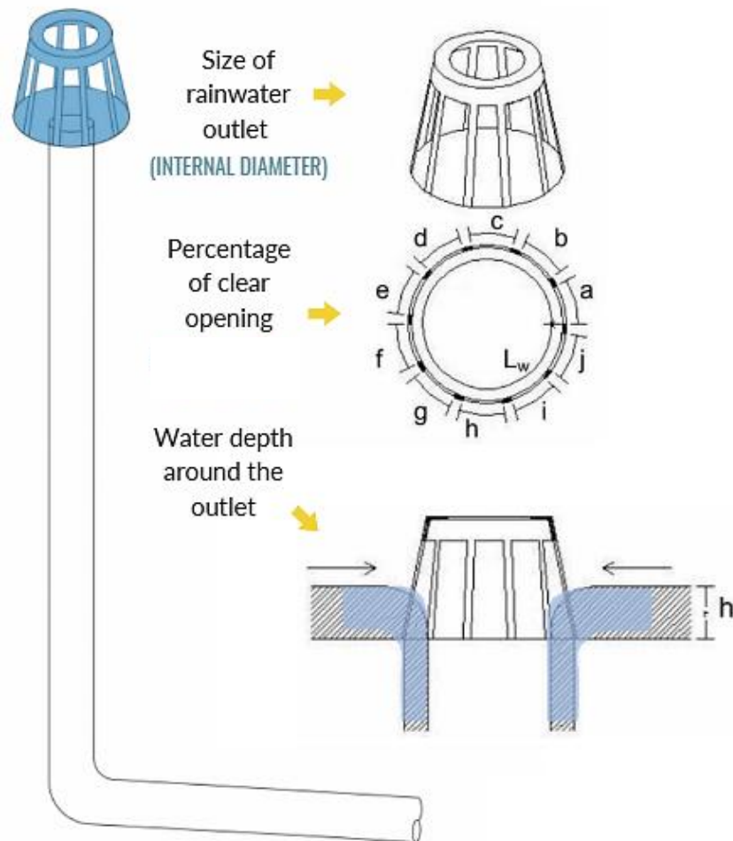
Figure 21: 3 Key Factors to Consider for the Rainwater Outlet Design
