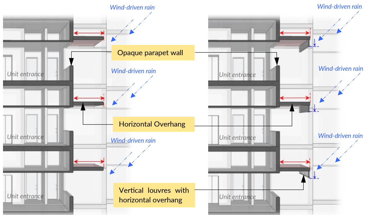
Figure 8: Provision of horizontal overhang and drop-down vertical louvres along corridors
