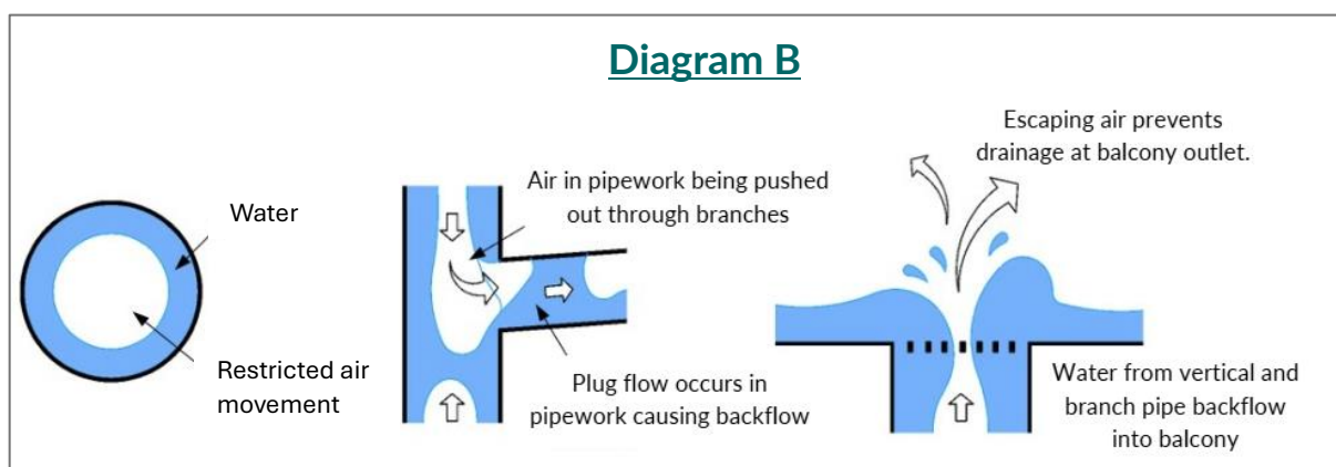
Figure 24: Under-Design of Balcony Drainage System causing Backflow
