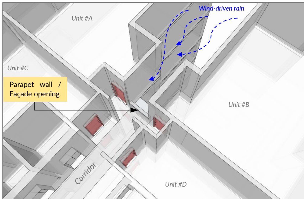
Figure 11: Diagram showing unit entrances (#A & #B) oriented away from façade opening
