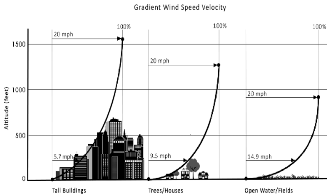
Figure 5: Variation of mean wind velocity profile with surface roughness (Extracted from Research Gate - Gherbi, Aboubakar & Belgasmia, Mourad. (2018))
