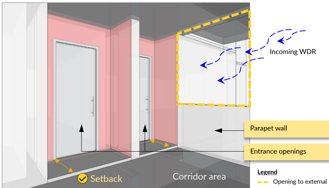
Figure 13: Residential Corridors with Recessed Unit Entrances Near Openings
