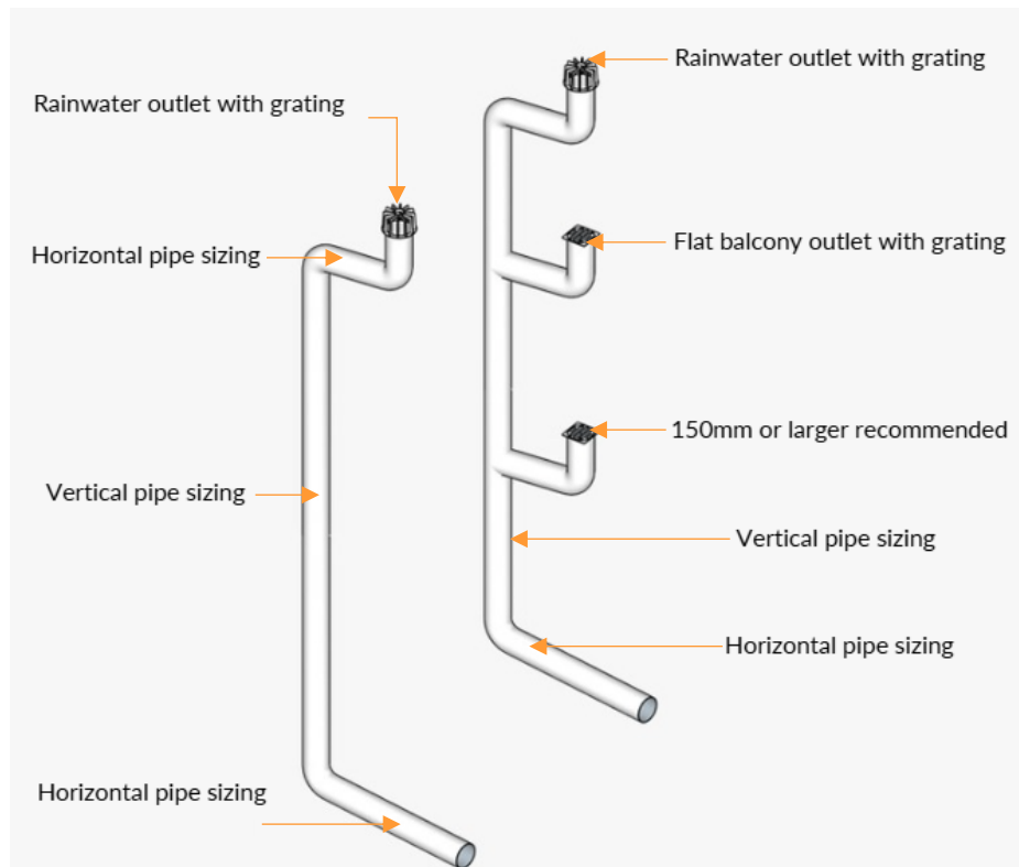
Figure 22: 3 Essential Components for Designing Effective Rainwater Drainage System
