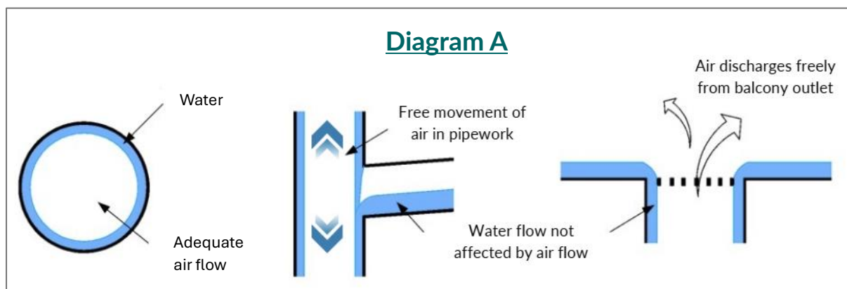
Figure 23: Correct Design of Balcony Drainage System
