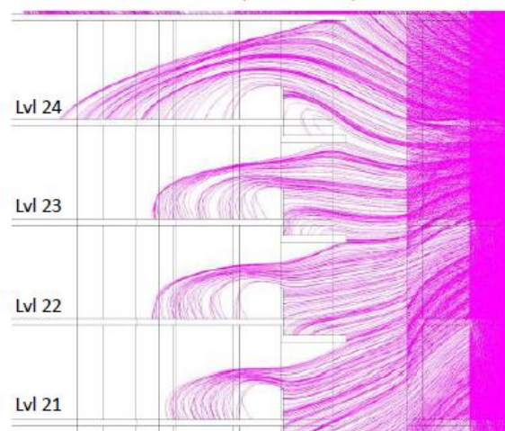
Figure 6: Wind-driven rain simulation showing more severe rainwater penetration at higher levels
