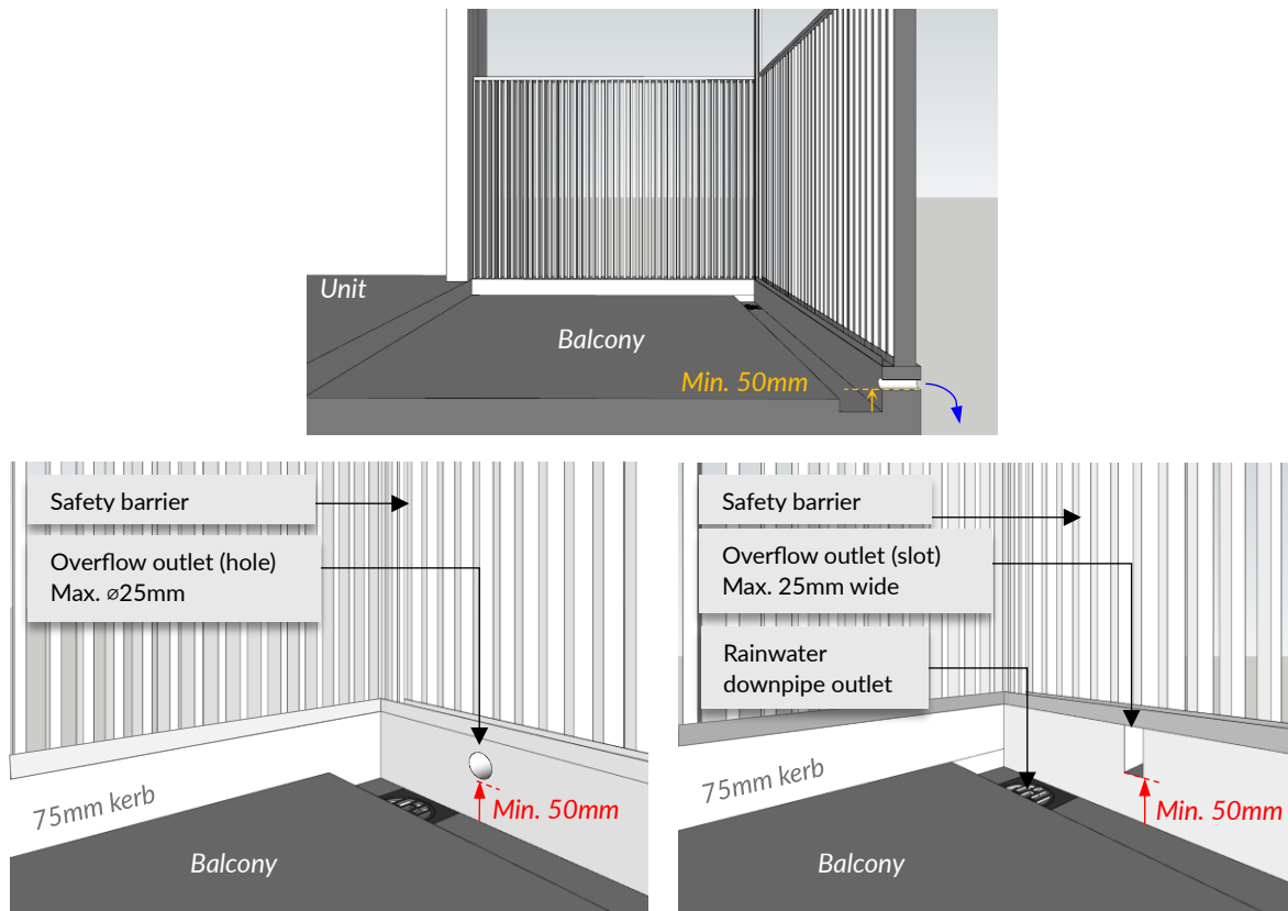
Figure 16: Balcony drainage system with overflow hole or slot as secondary measure to prevent flooding
