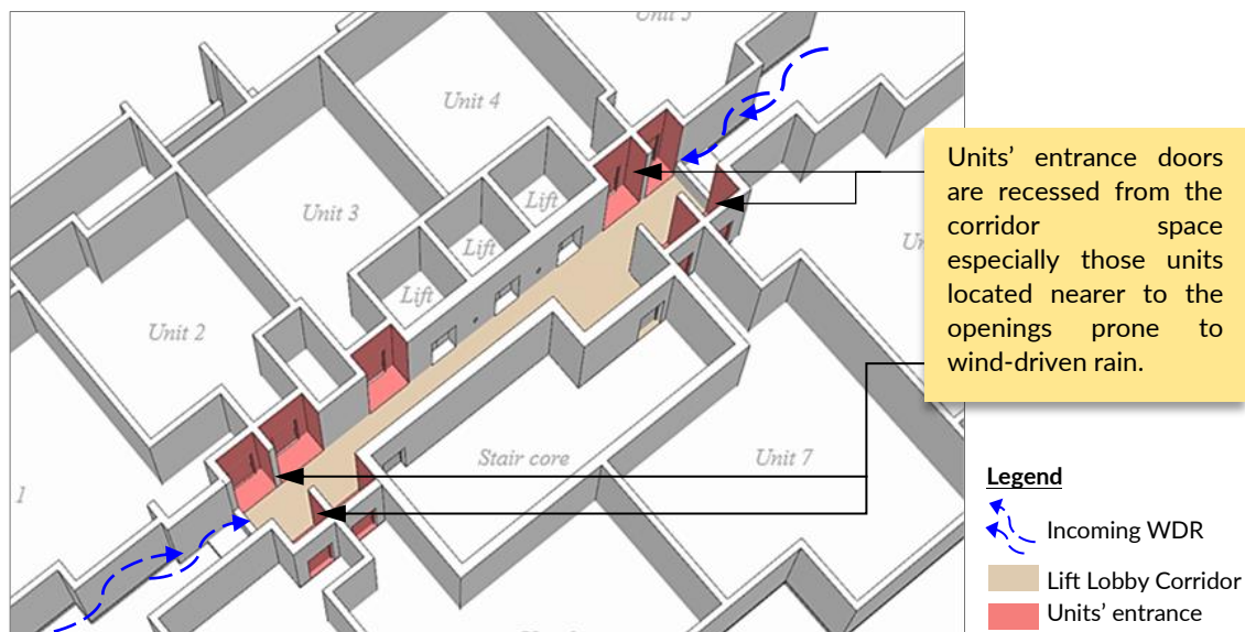
Figure 12: Diagram of Residential Corridor with Recessed Unit Entrances
