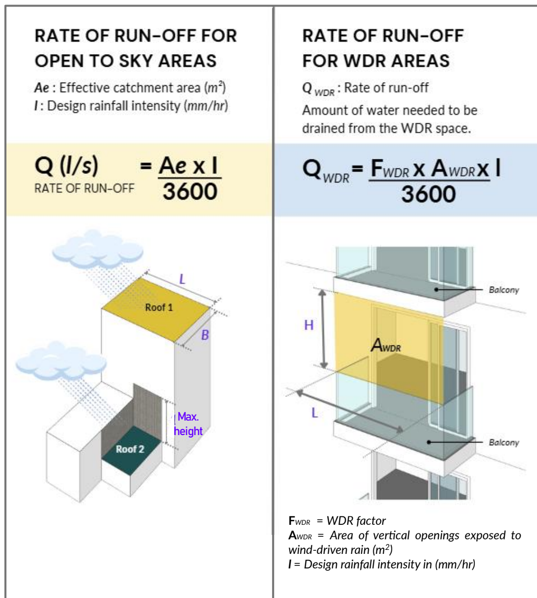
Figure 20: Comparison of run-off rate calculations for open-to-sky areas vs. wind-driven rain
