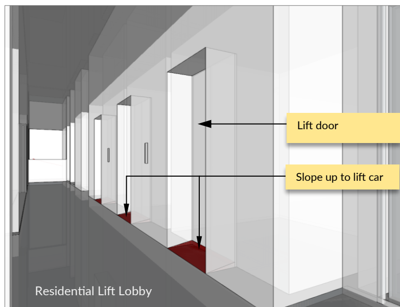
Figure 10: Residential Lift Lobby with Sloped Design to Prevent Rainwater Seepage
