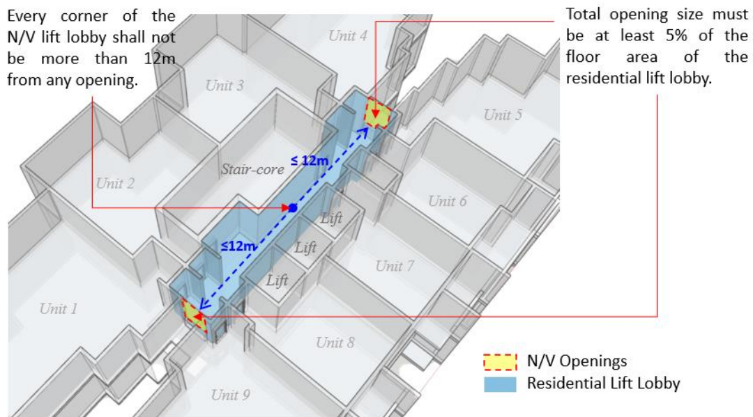
Figure 3: Provision of Natural Ventilation for Residential Lift Lobby
